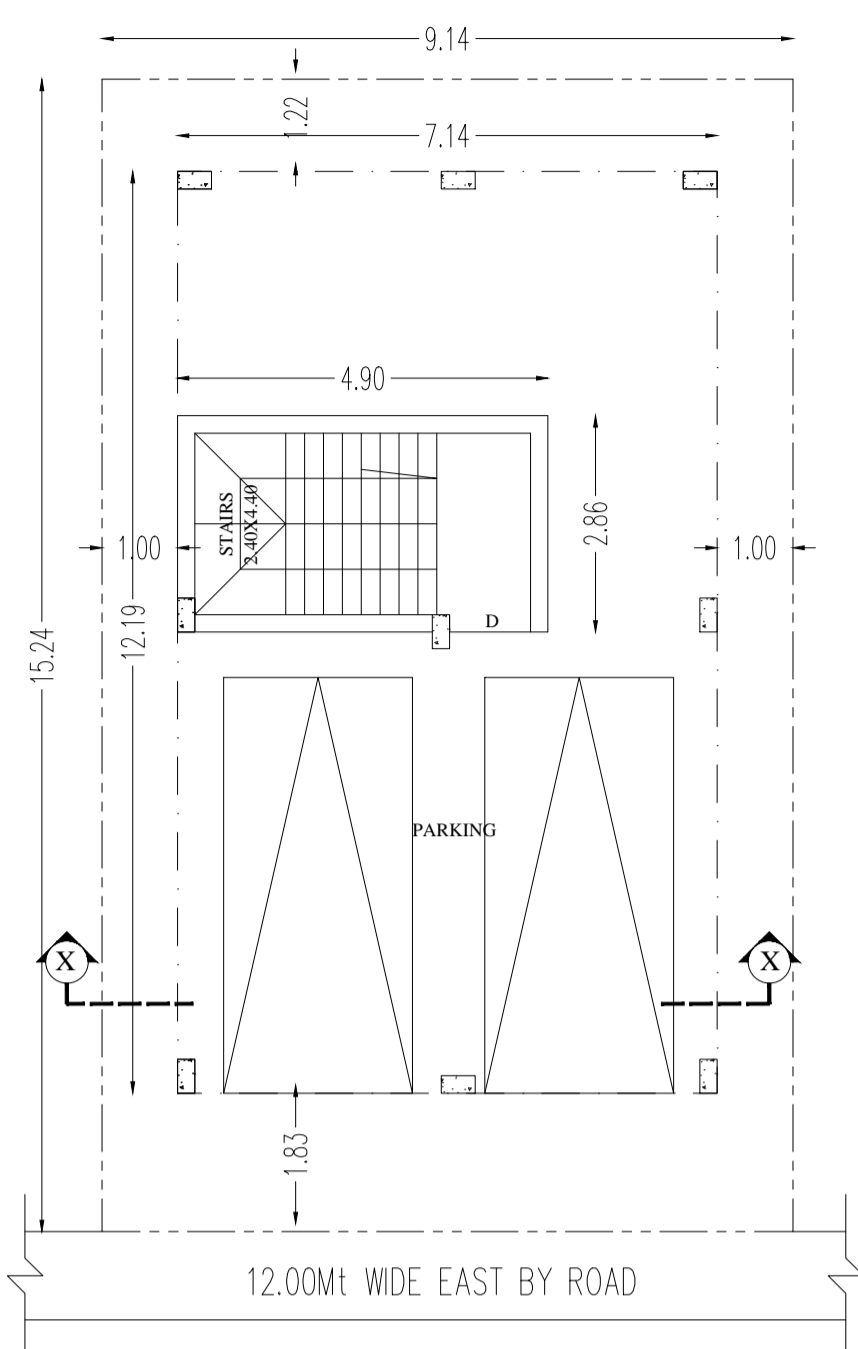
PROPOSED STILT FLOOR PLAN
